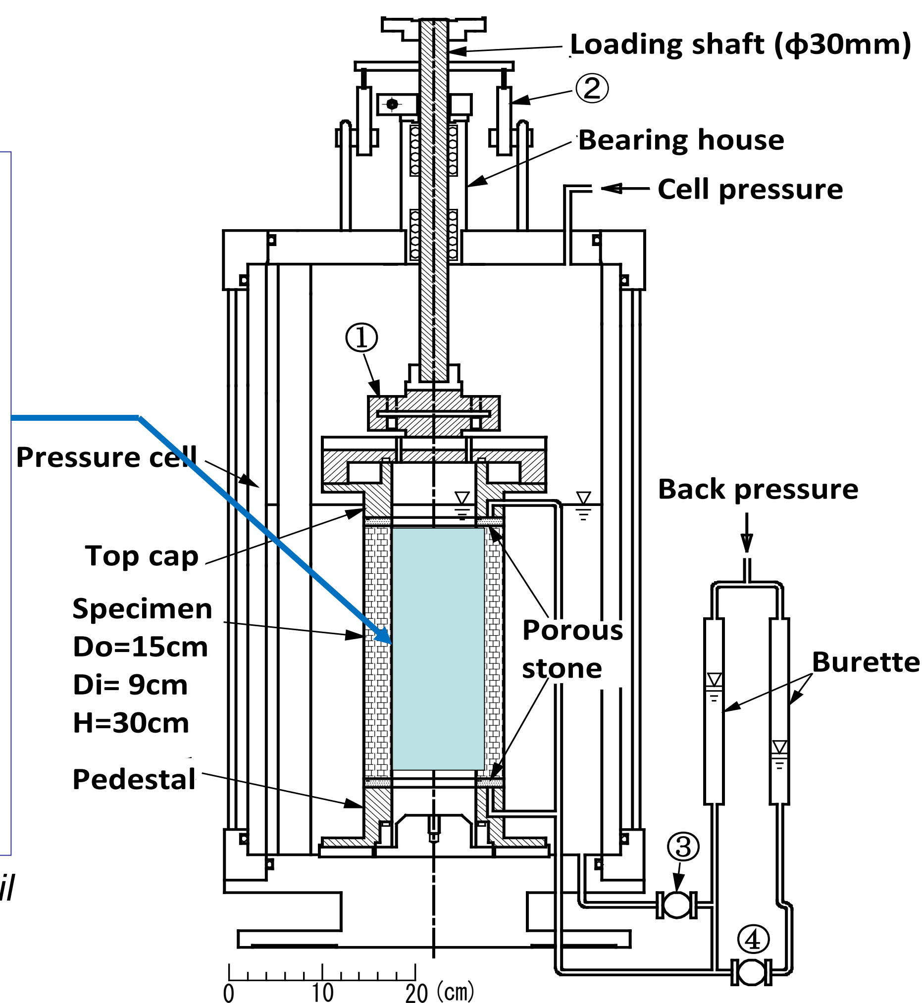
Fig. 2. Large-strain torsional shear apparatus used in this study
