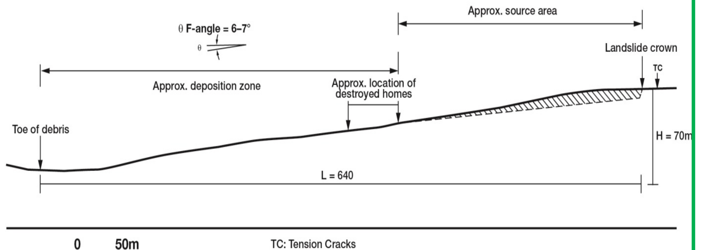
Fig. 3 Cross-section through the Takanodai landslide
