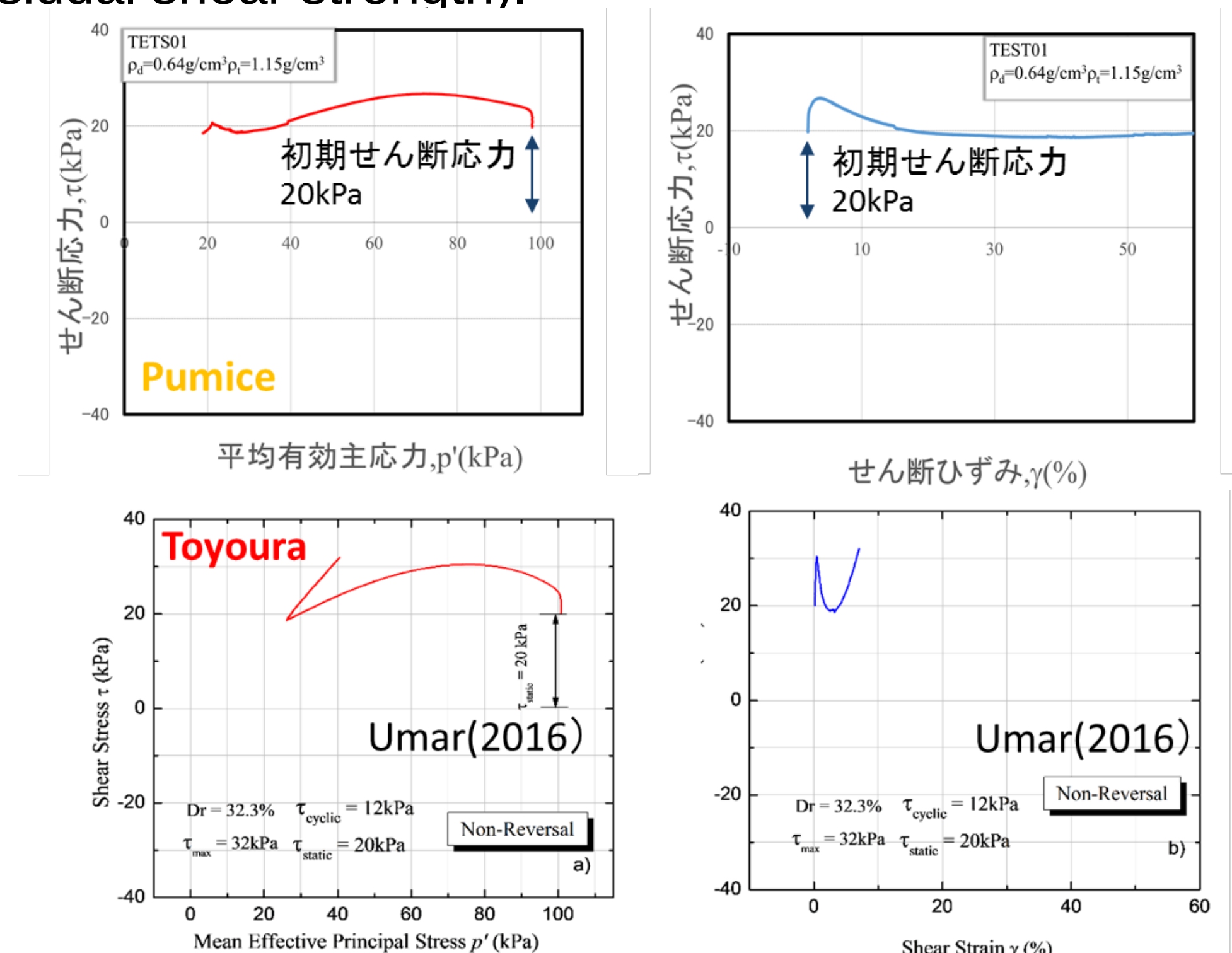
Fig. 6. Undrained monotonic test with initial static shear
